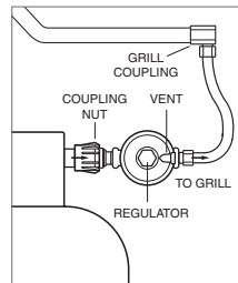
LP gas cylinder connection.
