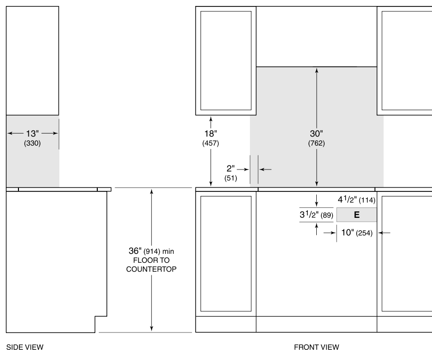
COUNTERTOP CUT-OUT
