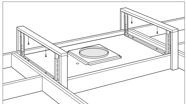
Hood installation
