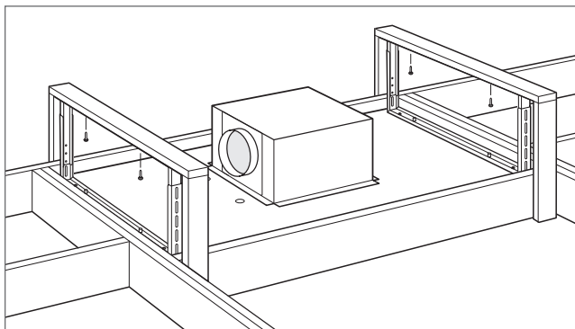
Hood installation
