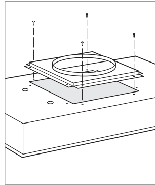
Flange installation
