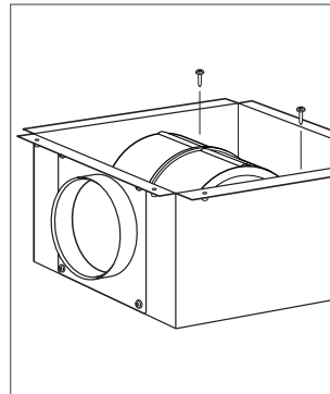
Internal blower installation
