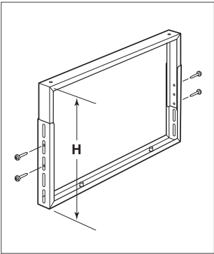
Bracket adjustment
